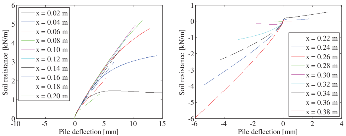
FIGURE 157. P-Y CURVES.
