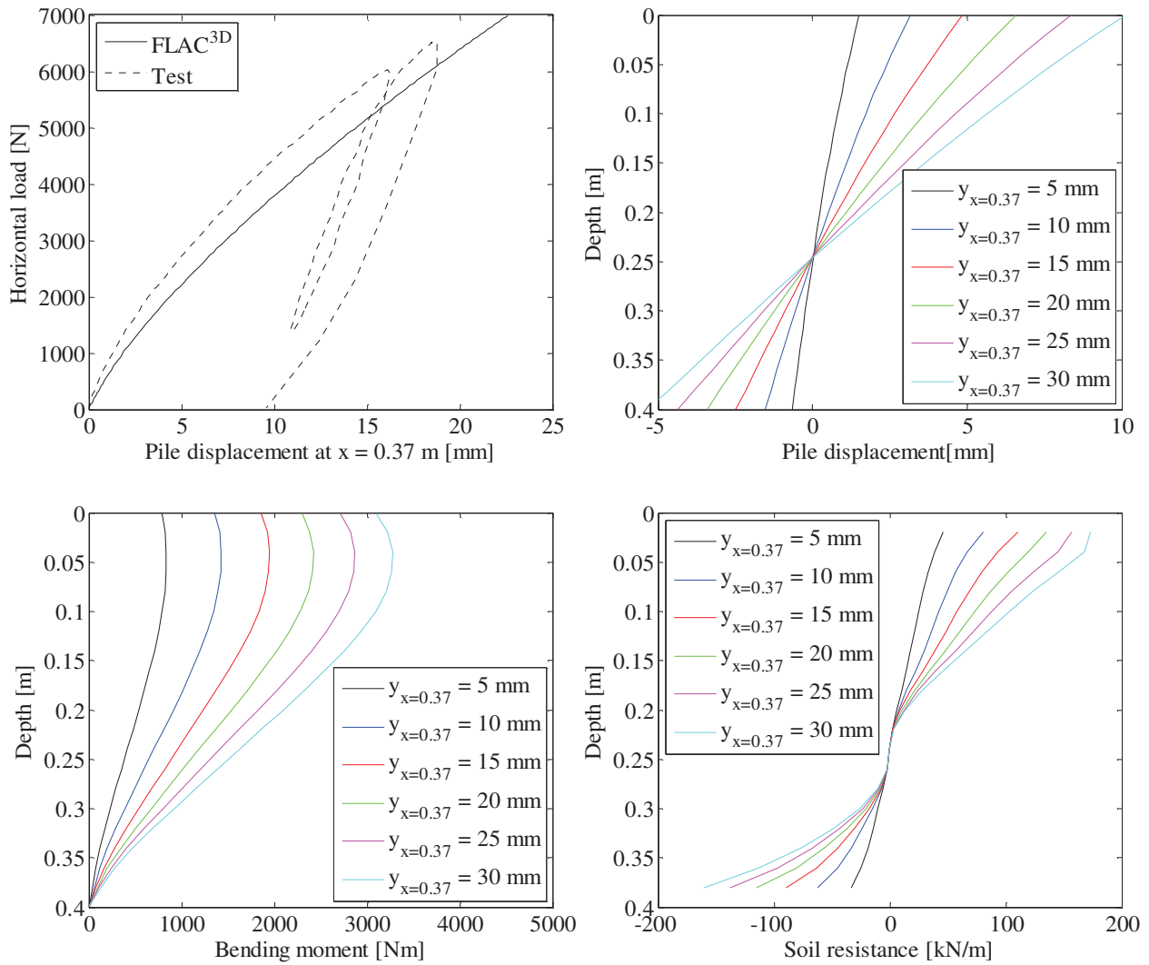
FIGURE 168. TOP LEFT: LOAD-DISPLACEMENT RELATIONSHIPS – TOP RIGHT: PILE DISPLACEMENT VERSUS DEPTH – BOTTOM LEFT: BENDING MOMENT VERSUS DEPTH – BOTTOM RIGHT: SOIL RESISTANCE VERSUS DEPTH.
