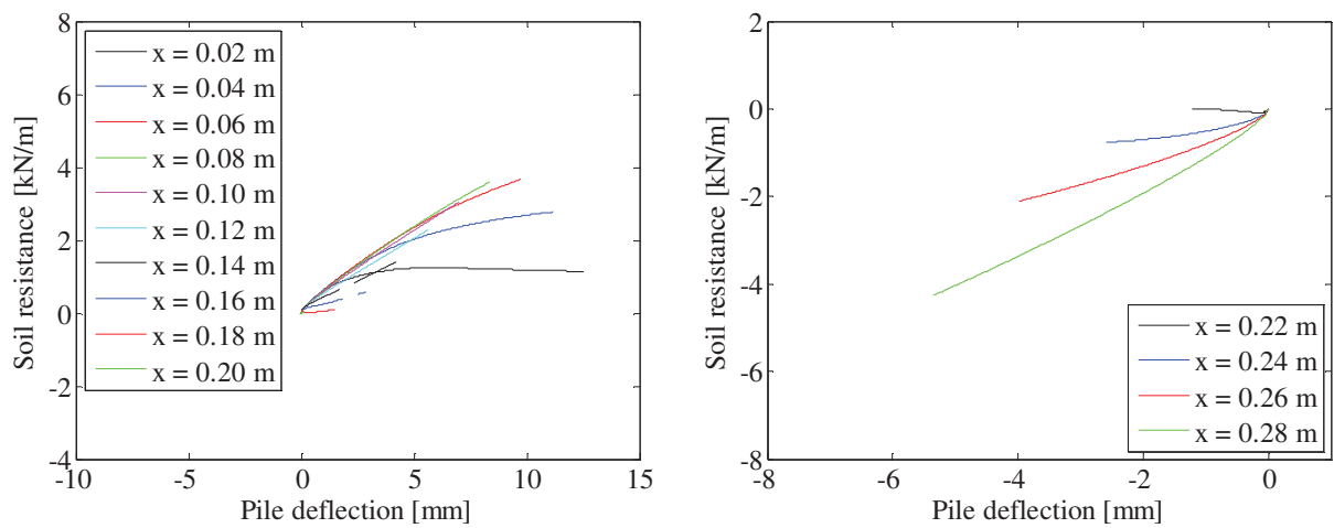
FIGURE 131. P-Y CURVES.
