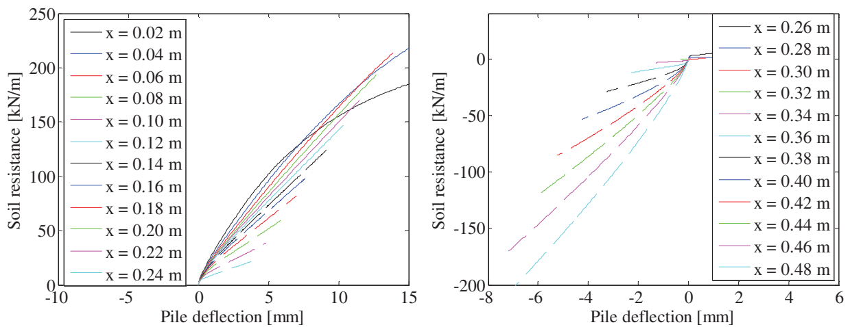
FIGURE 183. P-Y CURVES.
