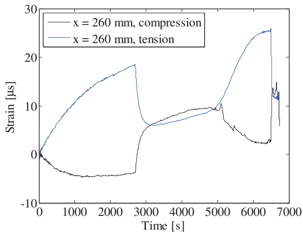
FIGURE 32. STRAIN GAUGE MEASUREMENTS.
