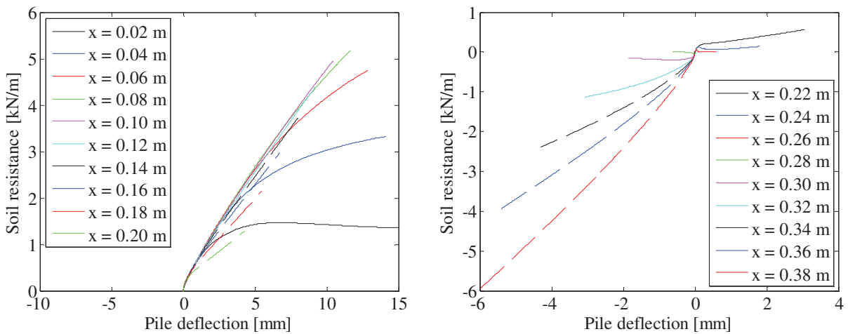
FIGURE 159. P-Y CURVES.
