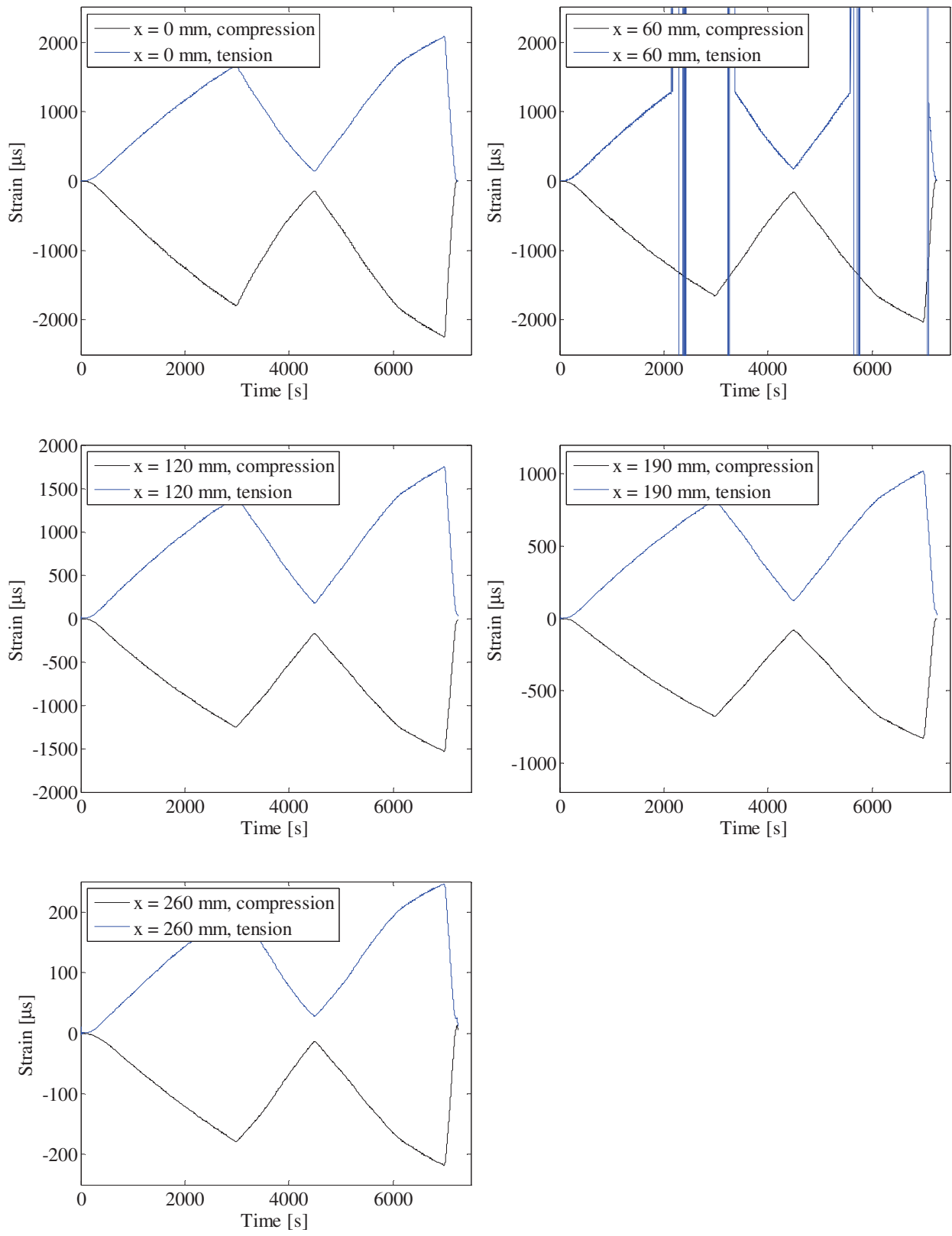
FIGURE 40. STRAIN GAUGE MEASUREMENTS.
