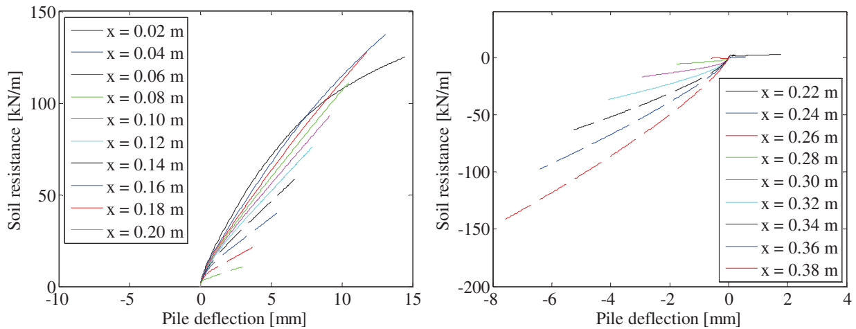
FIGURE 165. P-Y CURVES.
