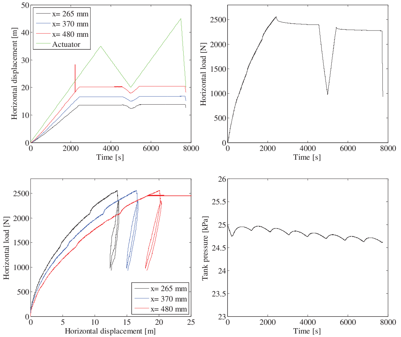
FIGURE 72. TOP LEFT: PILE DISPLACEMENT VERSUS TIME – TOP RIGHT: HORIZONTAL LOAD VERSUS TIME – BOTTOM LEFT: HORIZONTAL LOAD VERSUS PILE DISPLACEMENT – BOTTOM RIGHT: TANK PRESSURE VERSUS TIME.
