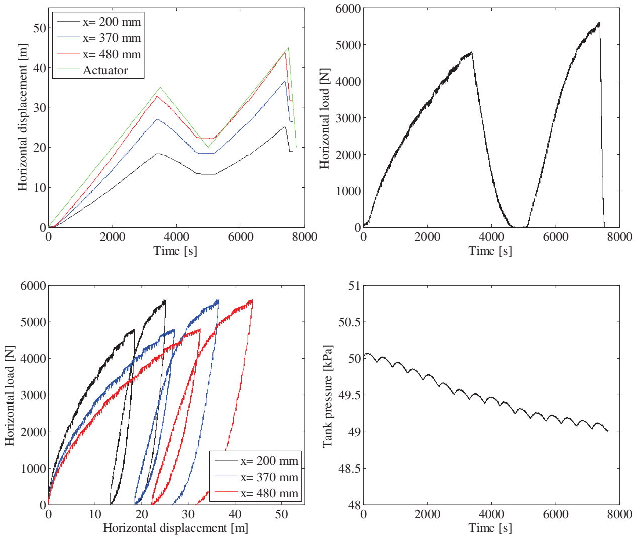
FIGURE 53. TOP LEFT: PILE DISPLACEMENT VERSUS TIME – TOP RIGHT: HORIZONTAL LOAD VERSUS TIME – BOTTOM LEFT: HORIZONTAL LOAD VERSUS PILE DISPLACEMENT – BOTTOM RIGHT: TANK PRESSURE VERSUS TIME.
