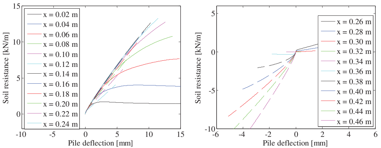
FIGURE 175. P-Y CURVES.
