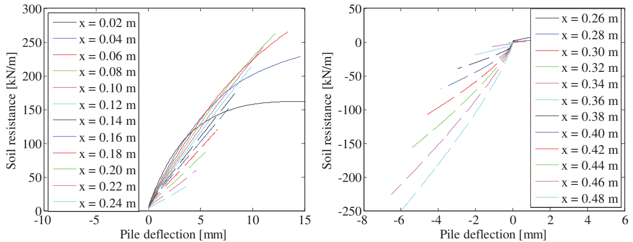
FIGURE 187. P-Y CURVES.
