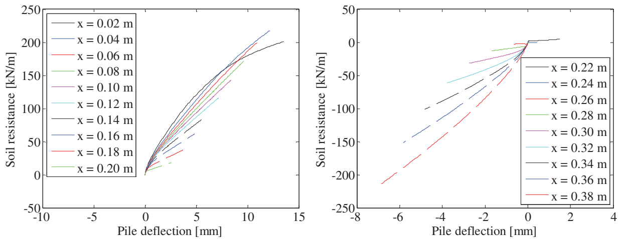
FIGURE 169. P-Y CURVES.
