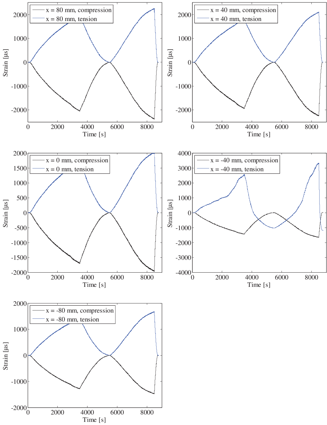
FIGURE 109. STRAIN GAUGE MEASUREMENTS.
