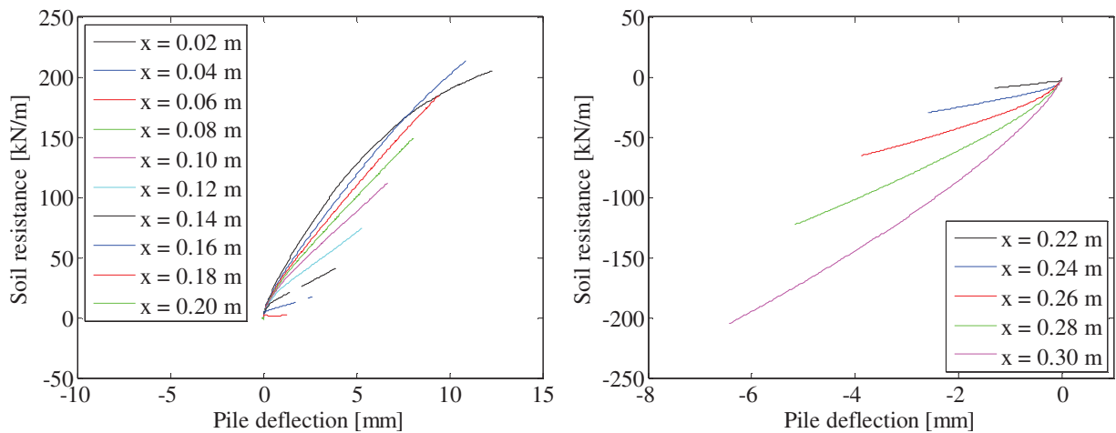
FIGURE 155. P-Y CURVES.
