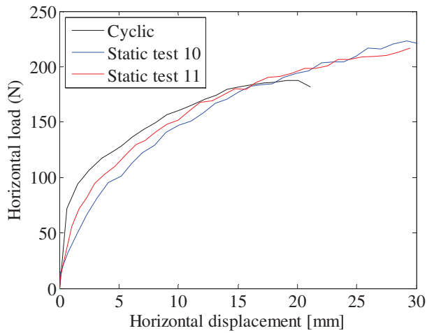
FIGURE 31. COMPARISON OF THE LOAD-DISPLACEMENT RELATIONSHIP FROM THE CYCLIC TESTS WITH THE QUASI-STATIC TESTS. D = 80 \text{ mm} , L_p = 320 \text{ mm} , P_0 = 0 \text{ kPa} .
