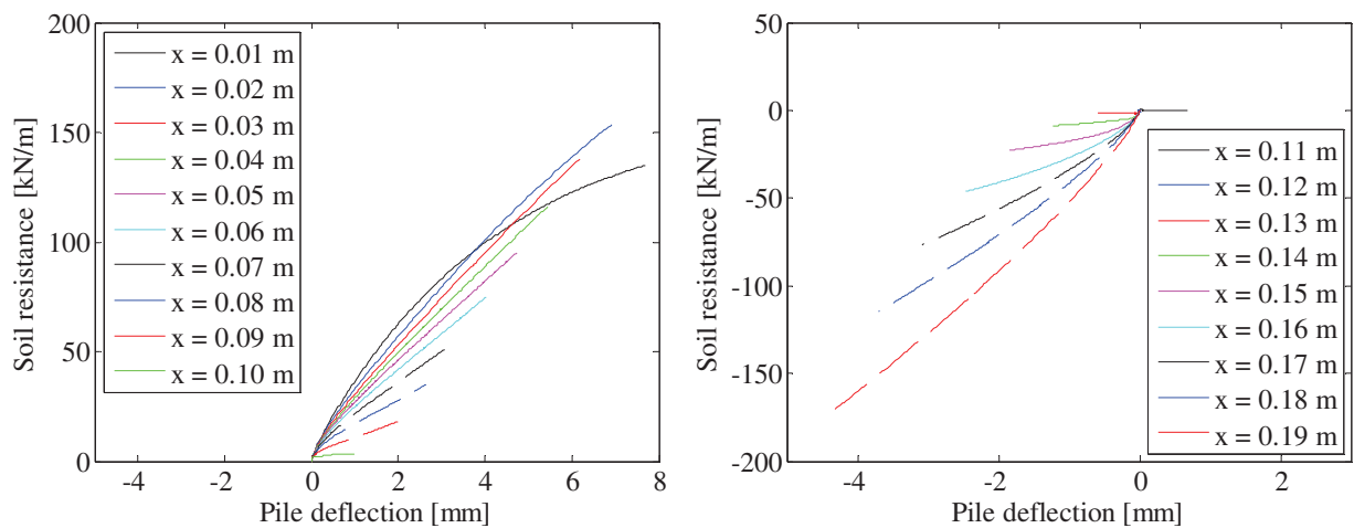
FIGURE 129. P-Y CURVES.
