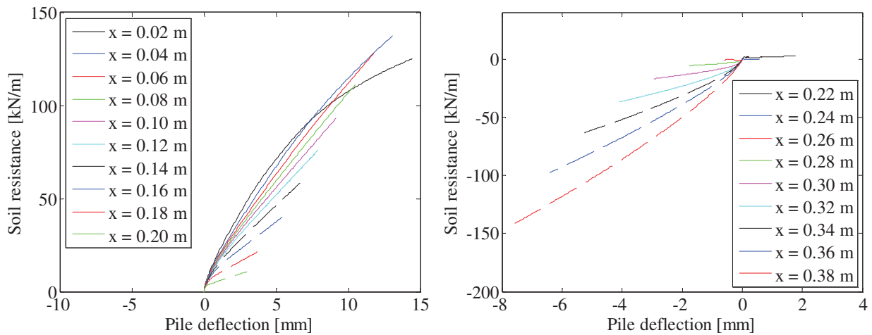
FIGURE 163. P-Y CURVES.
