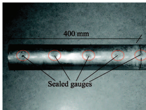
FIGURE 9. STRAIN GAUGES INSTALLED ON THE 80 MM PILE WITH STRAIN GAUGES ATTACHED IN 5 LEVELS. THE GAUGES ARE INSTALLED IN MILLED GROOVES.
