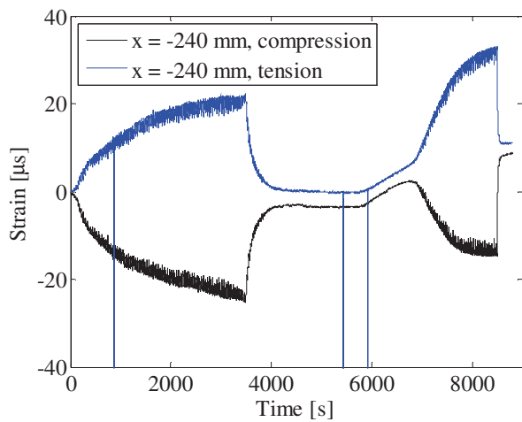
FIGURE 50. STRAIN GAUGE MEASUREMENTS.
