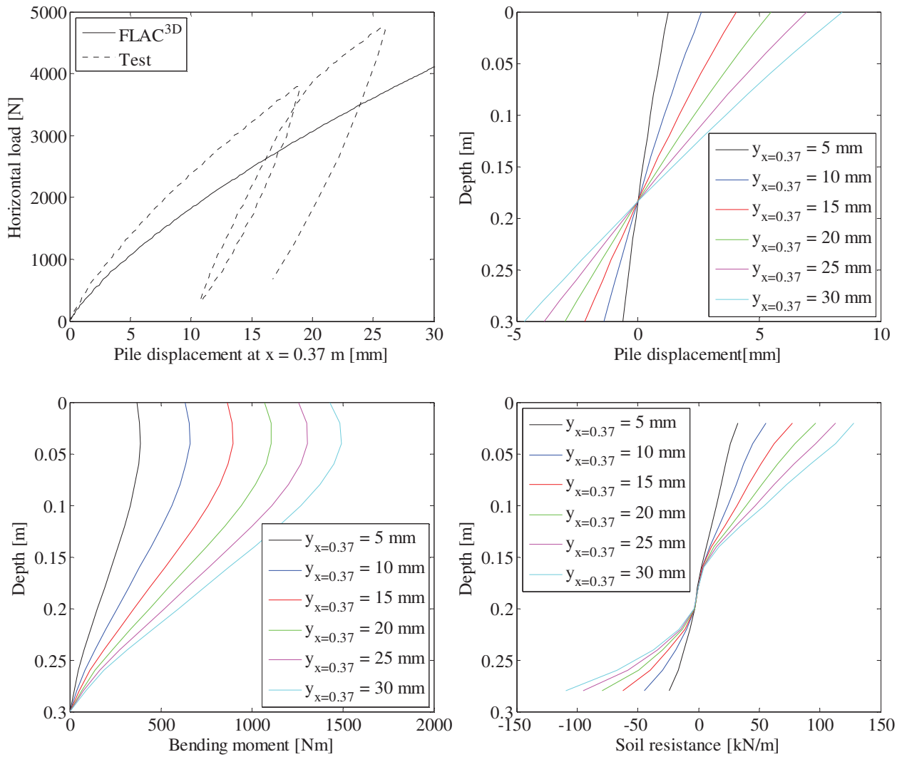
FIGURE 134. TOP LEFT: LOAD-DISPLACEMENT RELATIONSHIPS – TOP RIGHT: PILE DISPLACEMENT VERSUS DEPTH – BOTTOM LEFT: BENDING MOMENT VERSUS DEPTH – BOTTOM RIGHT: SOIL RESISTANCE VERSUS DEPTH.
