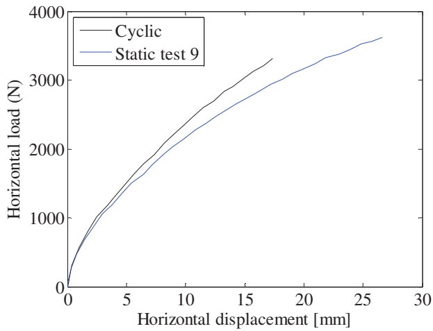
FIGURE 30. COMPARISON OF THE LOAD-DISPLACEMENT RELATIONSHIP FROM THE CYCLIC TESTS WITH THE QUASI-STATIC TESTS. D = 80 \text{ mm} , L_p = 240 \text{ mm} , P_0 = 100 \text{ kPa} .
