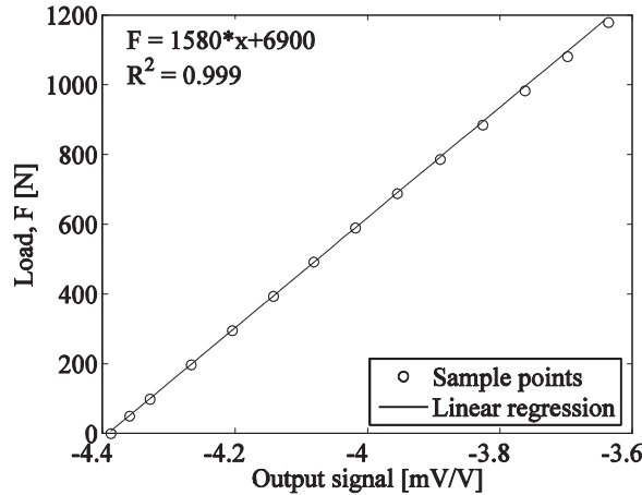
FIGURE 20. RESULTS FROM ONE THE CPT-CALIBRATIONS.
