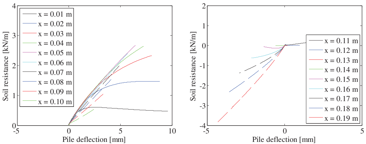
FIGURE 125. P-Y CURVES.
