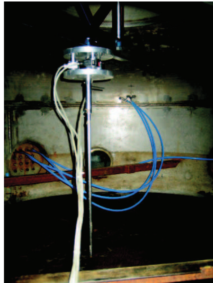
FIGURE 16. PICTURE FROM A CPT-TEST.
