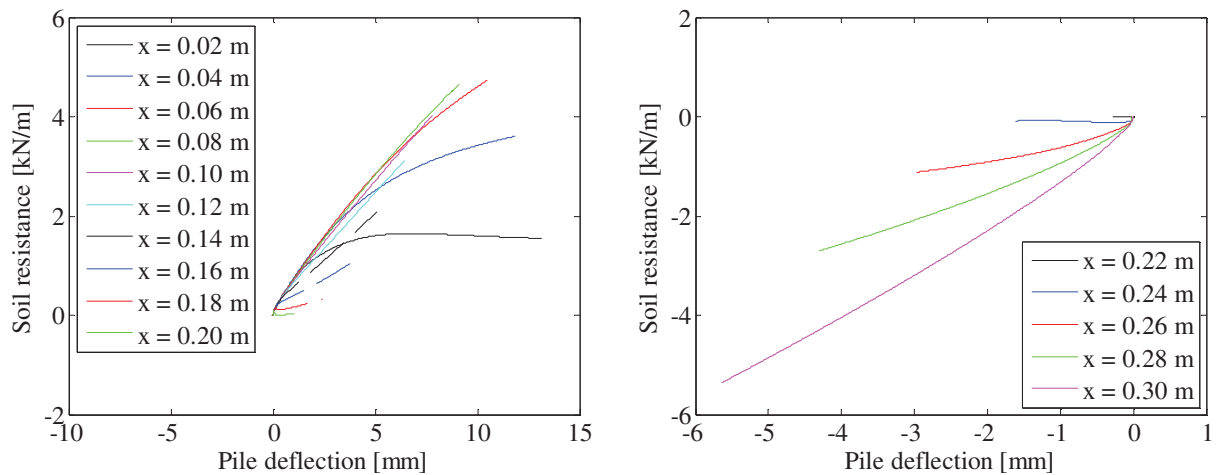
FIGURE 151. P-Y CURVES.
