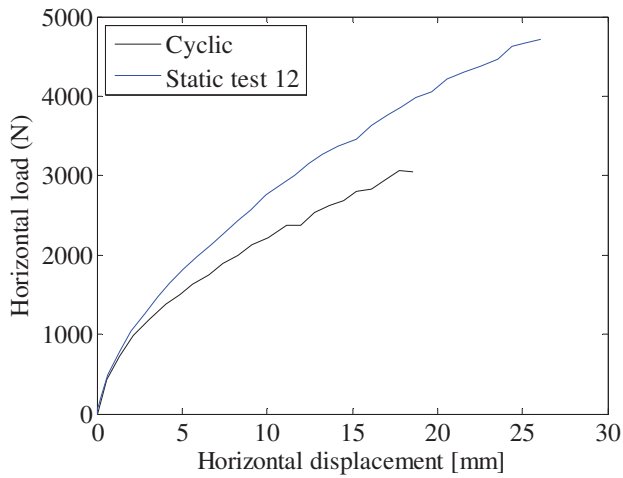
FIGURE 32. COMPARISON OF THE LOAD-DISPLACEMENT RELATIONSHIP FROM THE CYCLIC TESTS WITH THE QUASI-STATIC TESTS. D = 80 \text{ mm} , L_p = 320 \text{ mm} , P_0 = 50 \text{ kPa} .
