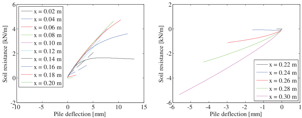
FIGURE 149. P-Y CURVES.
