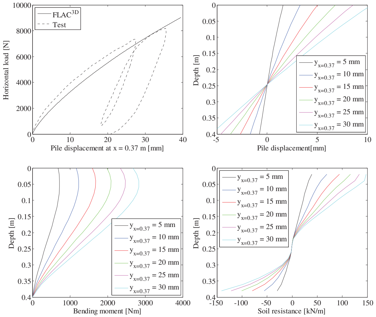
FIGURE 166. TOP LEFT: LOAD-DISPLACEMENT RELATIONSHIPS – TOP RIGHT: PILE DISPLACEMENT VERSUS DEPTH – BOTTOM LEFT: BENDING MOMENT VERSUS DEPTH – BOTTOM RIGHT: SOIL RESISTANCE VERSUS DEPTH.
