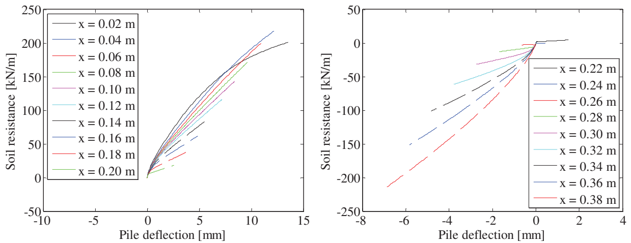
FIGURE 171. P-Y CURVES.
