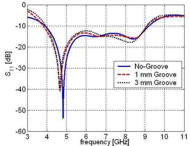
Fig. 1. The power reflection coefficient versus groove size. Every figure caption should be fully justified and end with a period. Use 10 pt font.
