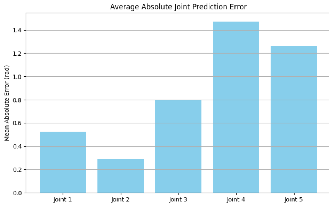
Fig. 13 Mean absolute error (MAE) per joint for the hybrid-trained model on real-image test data.
