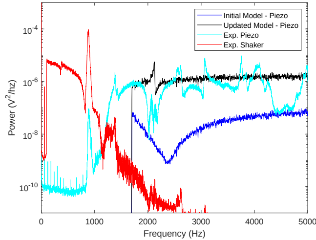
Fig. 21 Comparison between auto power spectra of Piezo and Shaker voltage of the experiment and models for an environment of 0.001 \text{ g}^2/\text{Hz} . Voltage powers are calculated from the control signals before amplification.
