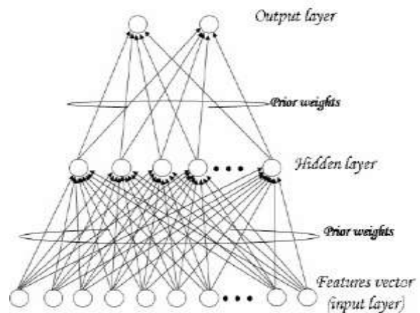
Fig. 1 BNN Architecture
