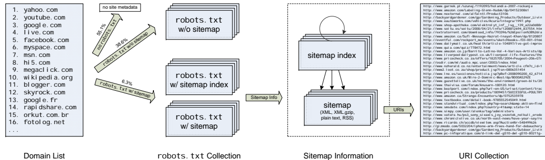
Fig. 8. Overview of the Crawling Process
