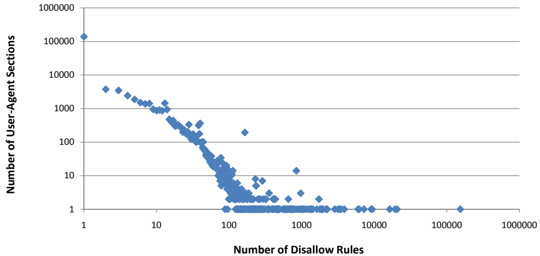
Fig. 6. Disallow Rules per User-Agent Section
