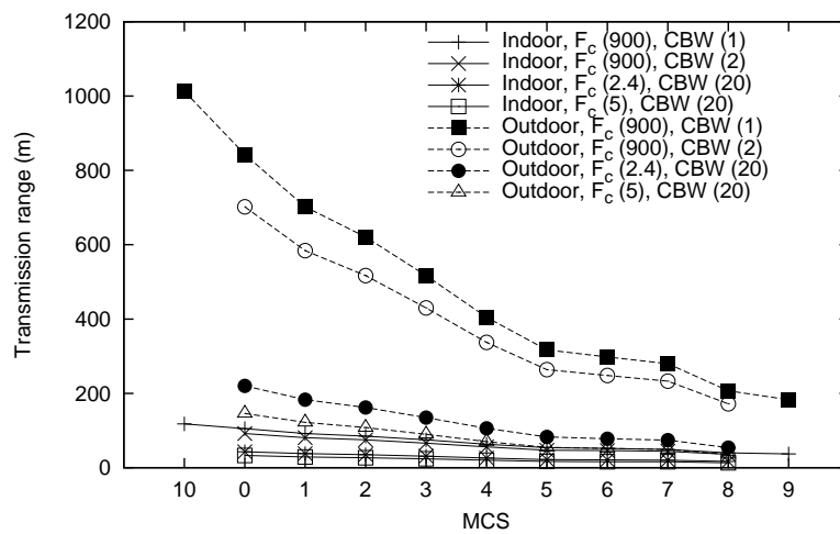
Figure 1 Comparison of transmission ranges with transmission power of 200 mW.
