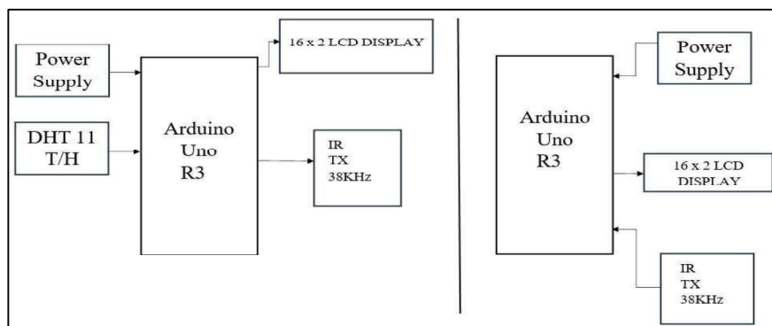
Fig1. UWOC Block diagram
