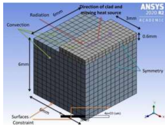
Figure 4. Geometry of 3-D model showing with thermal loading and boundary conditions
