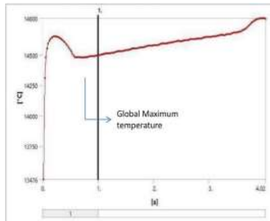
Figure 12. Global maximum temperature by FEM
