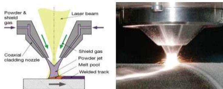
Figure 1. Laser Cladding Process 3
