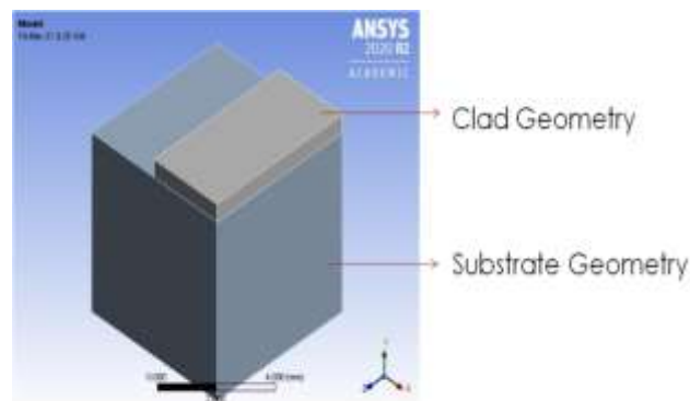
Figure 2. Geometry of the 3-D model
